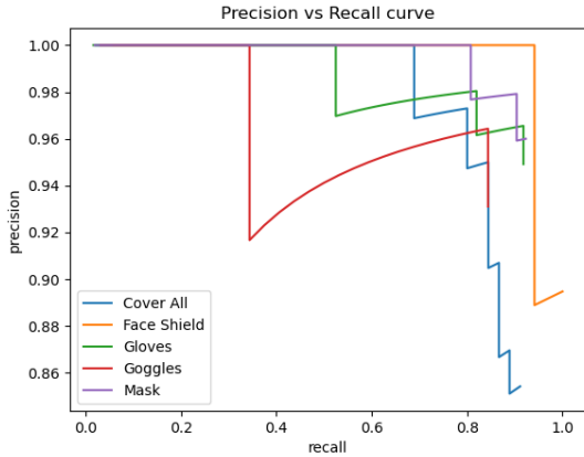
FIGURE 1. Precision-Recall curves for each of the five MPPE classes.
